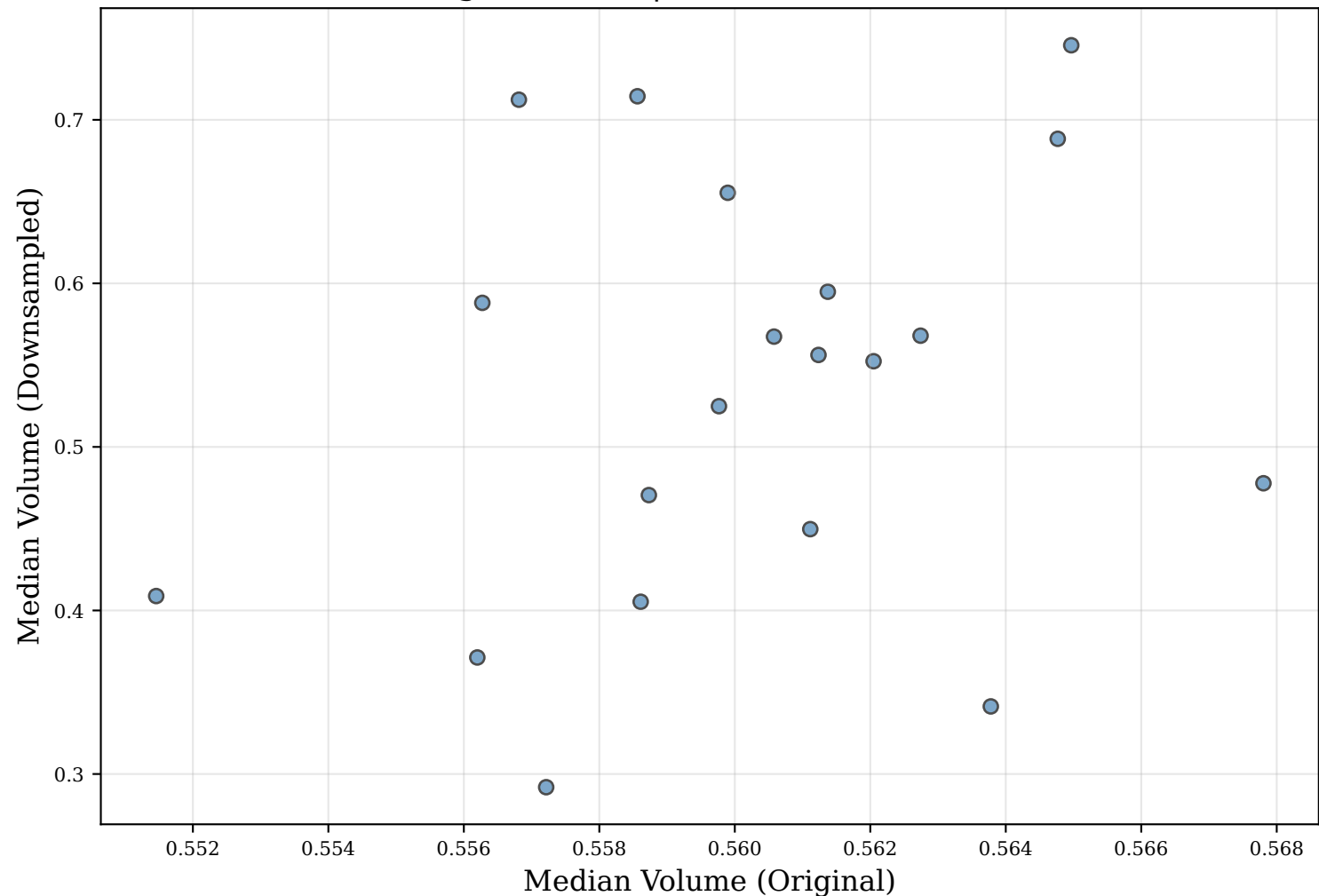
Median Volume: Original vs Downsampled sigma: (1, 1) | volume: (0.07, 0.9)
